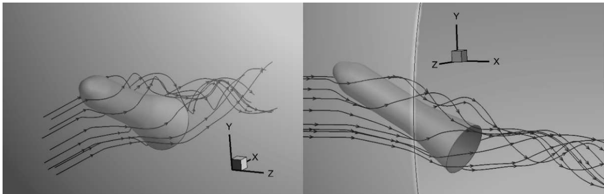
Spatial streamlines in modeling of the supersonic flow around the HB-2 model
